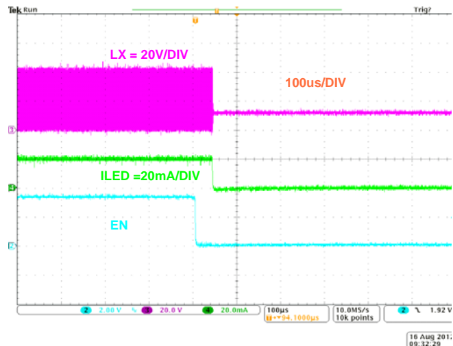
FIGURE 19. ISL97672B SHUTS DOWN AND STOPS SWITCHING \sim 30\mu s AFTER EN GOES LOW
